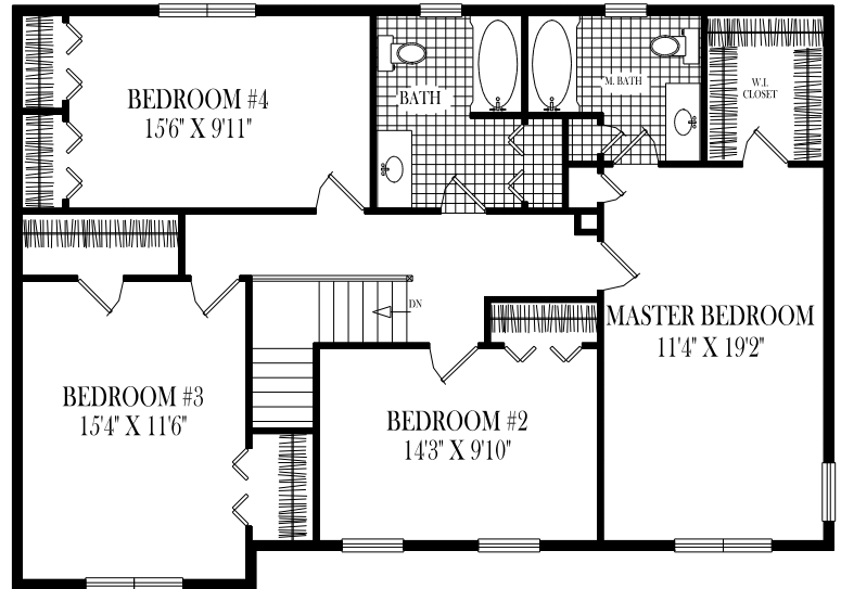
Optional Second Floor Plan
