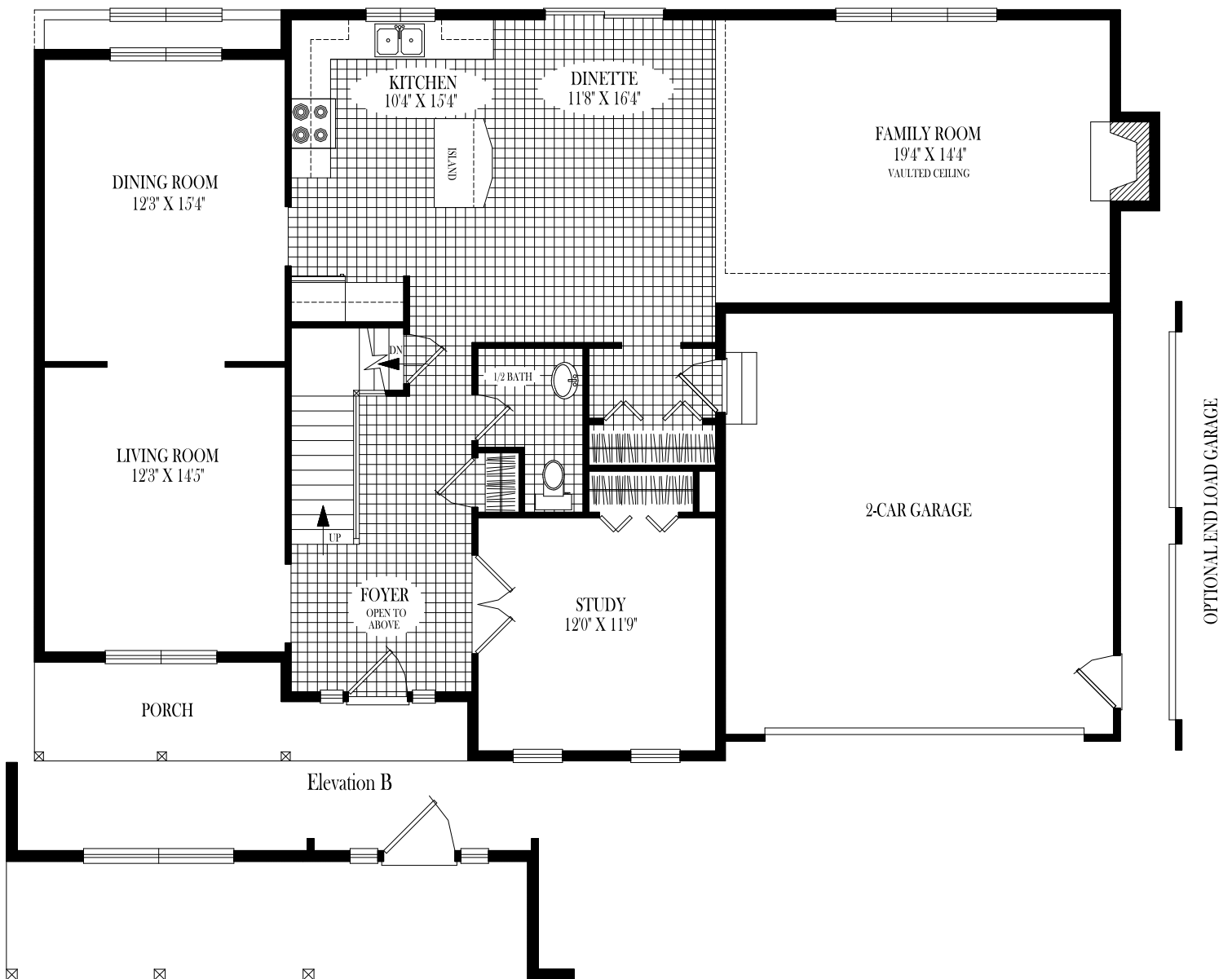
Rear Stair Option
